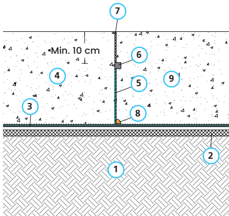
HORIZONTAL SECTION - VIEW FROM ABOVE
