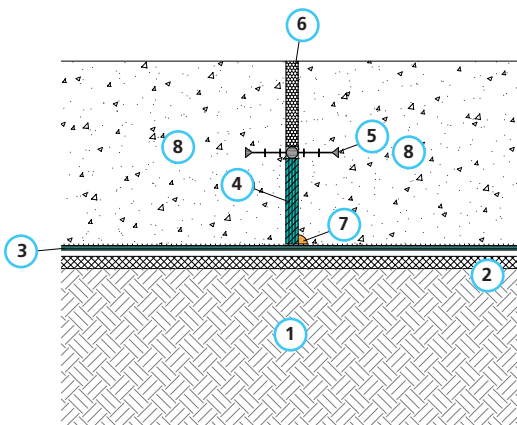
HORIZONTAL SECTION - VIEW FROM ABOVE
